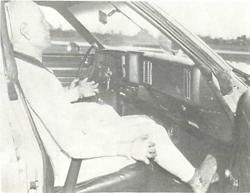
Figure 7-9 TEST NO. 1 – PRE AND POST INTERIOR VIEWS, CAR NO. 1 - CHEVELLE
