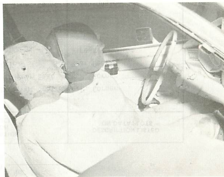
Figure 7-10 TEST NO. 1 – PRE AND POST INTERIOR VIEWS, CAR NO. 2 - PINTO
