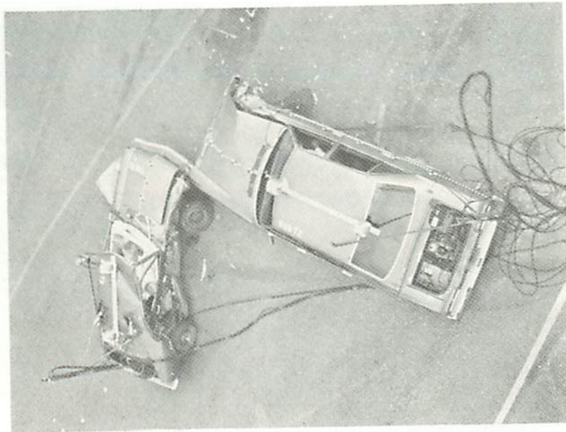
Figure 8-7 TEST NO. 2 – POST TEST COLLISION SCENE
