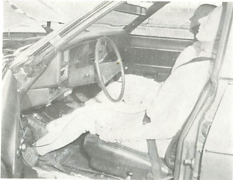
Figure 8-10 TEST NO. 2 – PRE AND POST INTERIOR VIEWS, CAR NO. 1 - CHEVELLE
