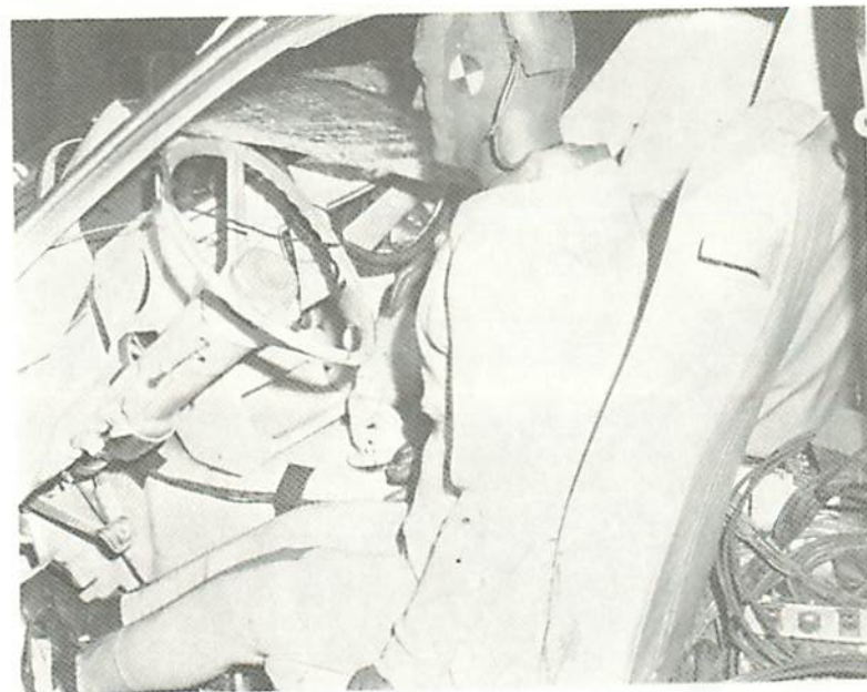
Figure 8-11 TEST NO. 2 – POST INTERIOR VIEW, CAR NO. 2 - PINTO
