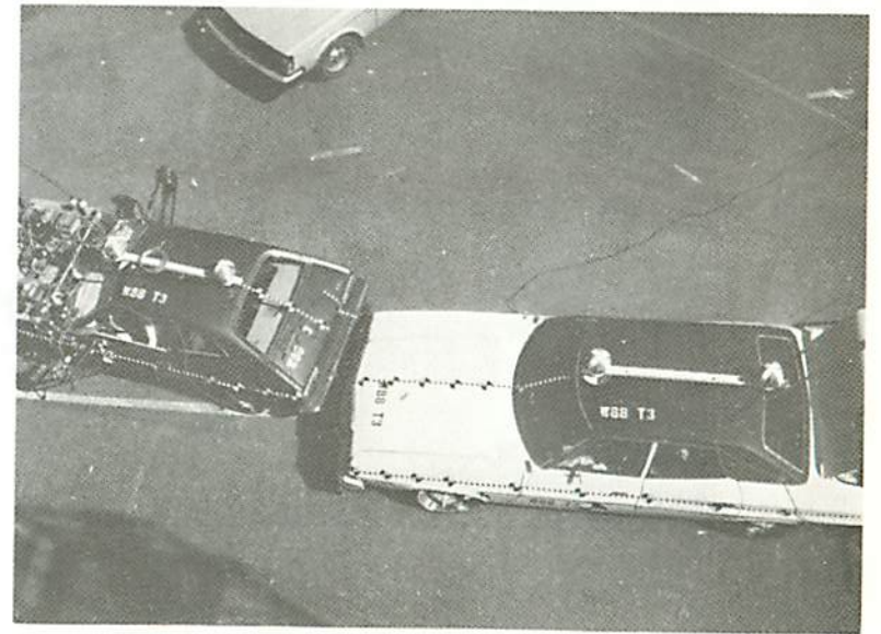
Figure 9-6 TEST NO. 3 – PRE TEST COLLISION CONFIGURATION
