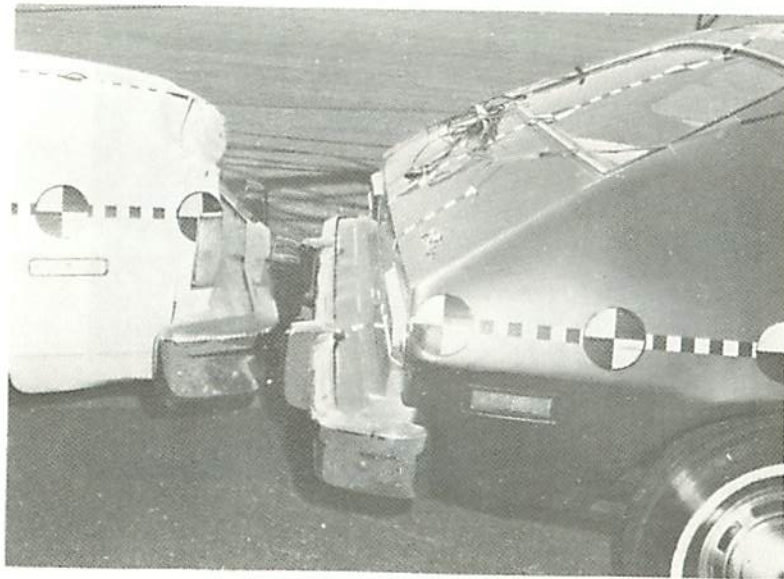
Figure 9-6 TEST NO. 3 – PRE TEST COLLISION CONFIGURATION
