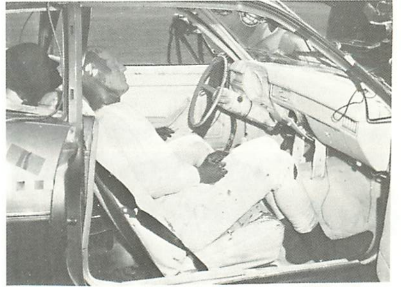
Figure 9-11 TEST NO. 3 – PRE AND POST INTERIOR VIEWS, CAR NO. 2 - PINTO
